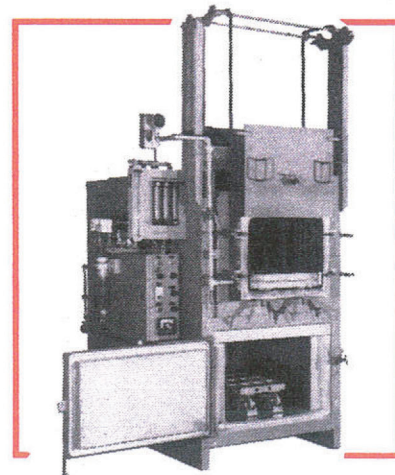
SERIES RETORT H&D MODEL 182538 WITH CARBURIZING PACKAGE
